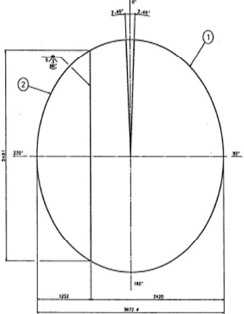
ARRANGEMENT OF ROOF PLATE
