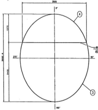
ARRANGEMENT OF BOTTOM PLATE
